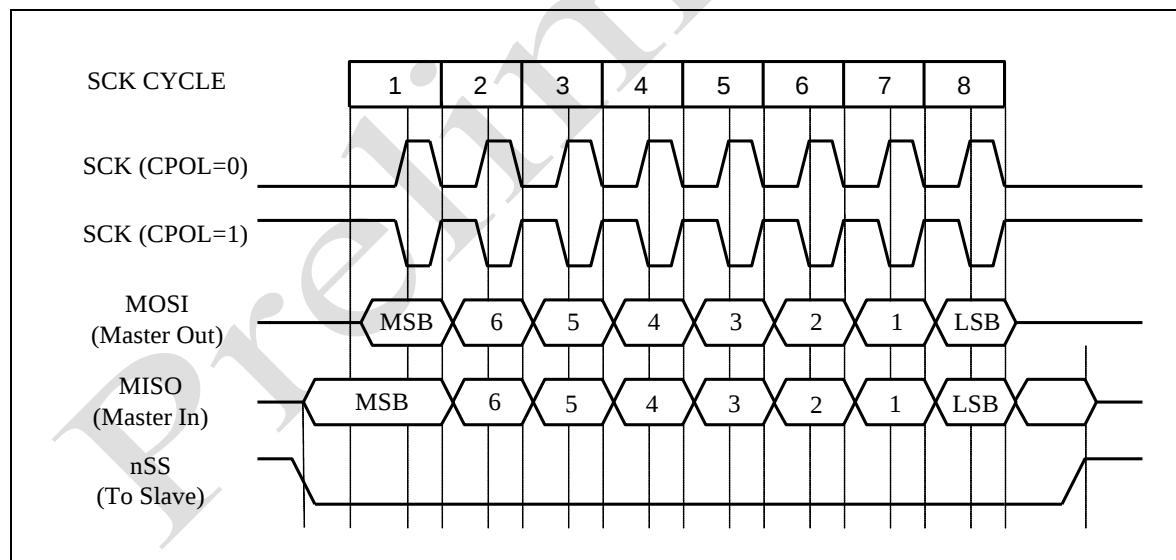
Figure 15-2 Transfer Timing when CPHA = '0'
