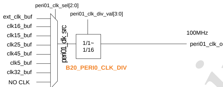
Figure 4-8 Peri Clock
