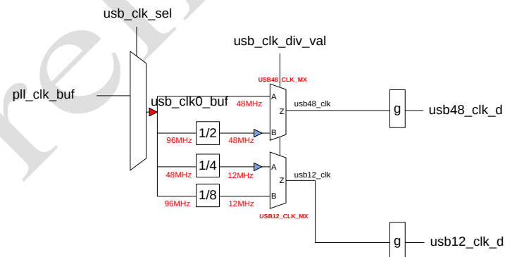
Figure 4-7 USB Clock
