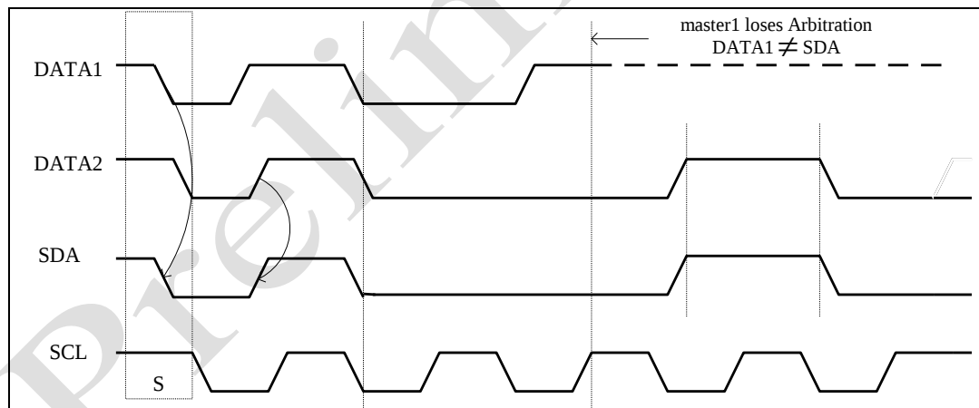
Figure 16-6 Bus arbitration 2
