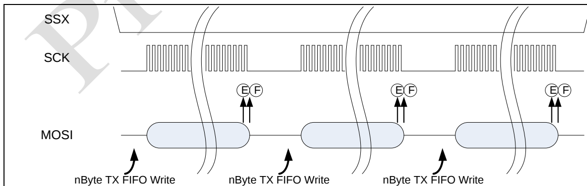
Figure 15-6 n-Bytes Transfer vs. Status and Interrupt
