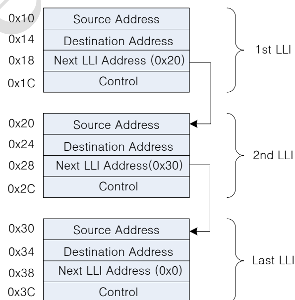
Figure 14-3 Linked list
