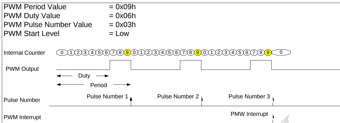
Figure 11-3 PWM Operation
