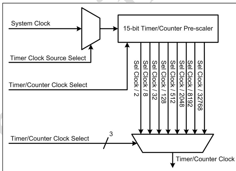
Figure 9-1 Pre-scaler Block Diagram
