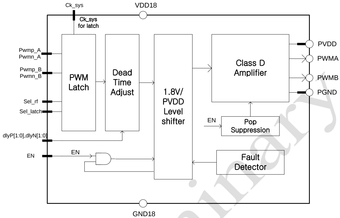
Figure 17-4 Speak Driver Block Diagram
