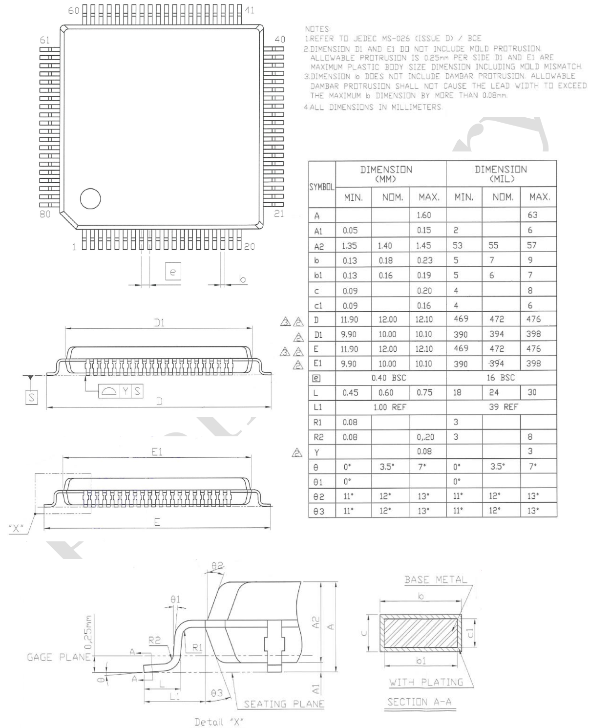
Figure 21-2 adLuna-TxxK Package Dimension
