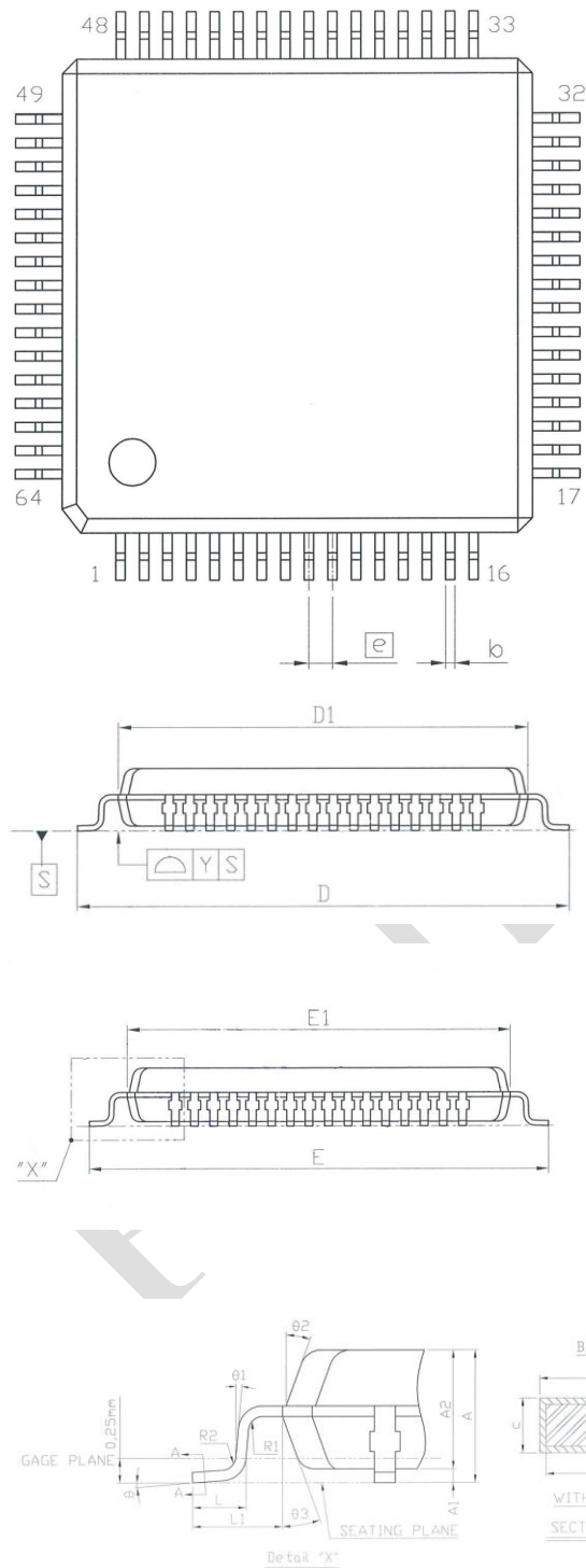
Figure 21-1 adLuna-TxxG Package Dimension
