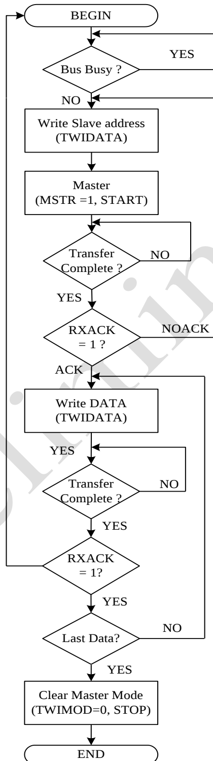
Figure 16-8 Master Transmit Flow Char
