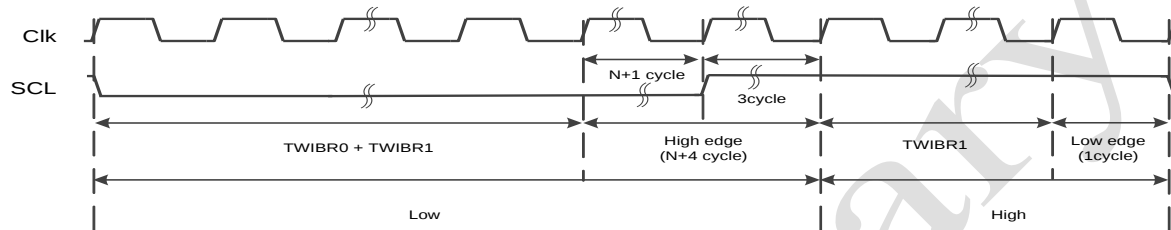
Figure 16-14 SCL Hold wave form
