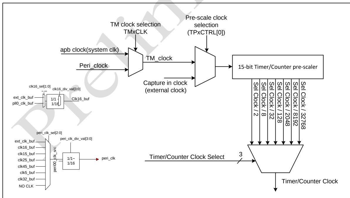
Figure 11-1 Pre-scaler Block Diagram
